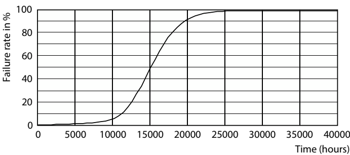
Life Expectancy Diagram - CorePro LED spot ND 7-50W MR16 827 36D
