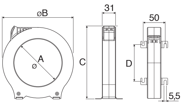
WGC 55, WGC 80, WGC 110, WGC 140, WGC 180 WGC-55-TB, WGC-80-TB, WGC-110-TB, WGC-140-TB, WGC-180-TB (mm)
