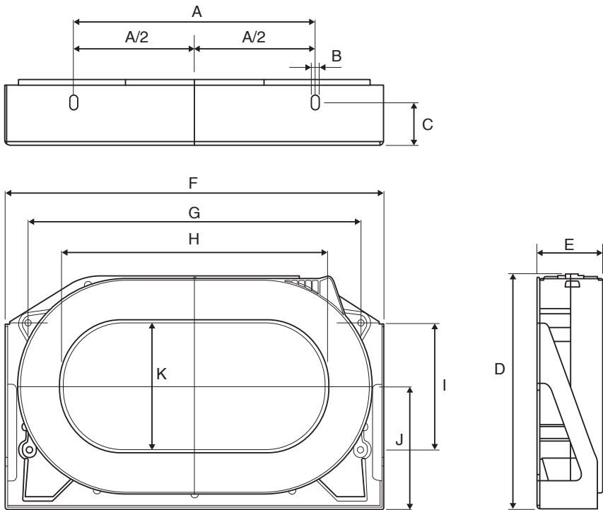
WGC 220x105, WGC 350x150, WGC 500x200 (mm)
