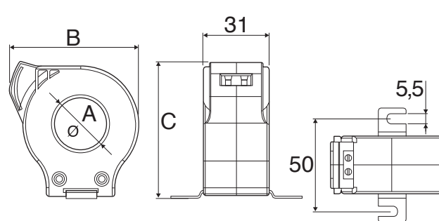
WGC 25, WGC 35, WGC-25-TB, WGC-35-TB (mm)
