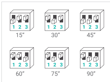
Flow switch mode (inhibition time)
