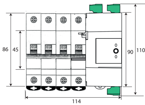
Instalación trifásica + neutro - 4 polos / Three-phase installation - 4 poles
