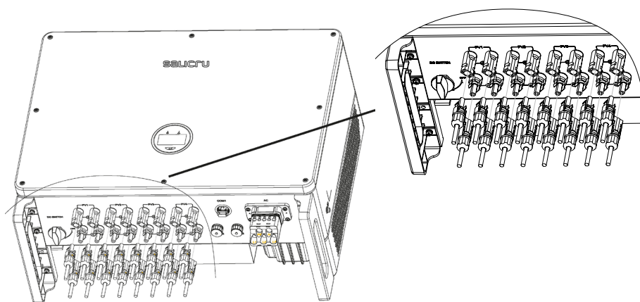
Fig. 31. Connecting the DC input terminals of units with 4 MPPTs.
