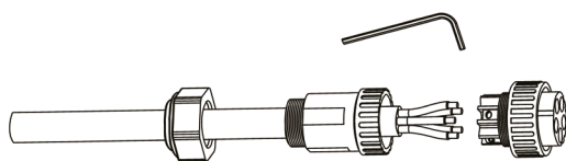
Fig. 35. Inserting the bare wire into the terminal.
