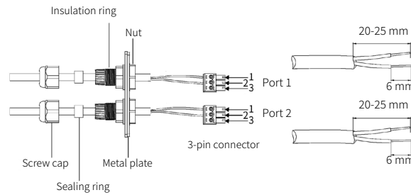
Fig. 41. Terminal connection process.
