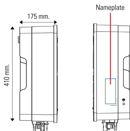
Fig. 3. Side view.
