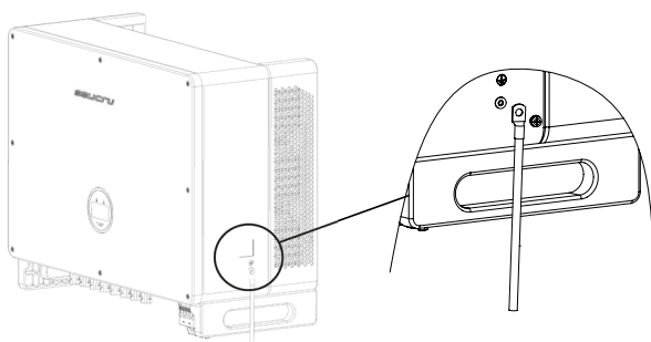
Fig. 20. Earthing terminal connection.
