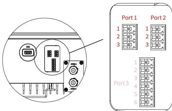
Fig. 40. Communication ports.
