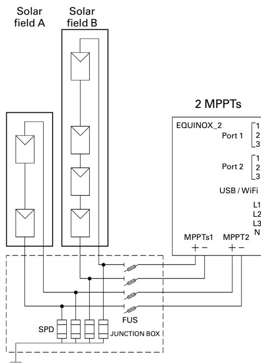
Fig. 28. Connection of several solar fields and 2 MPPTs.
