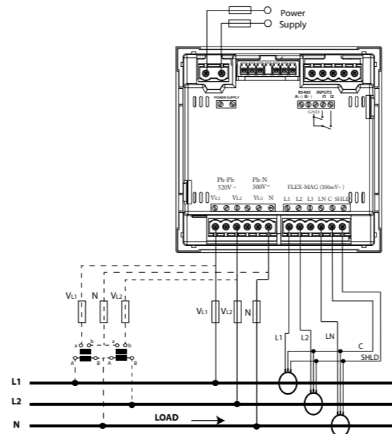
Red bifásica a 3 hilos / 3-wire two-phase network
