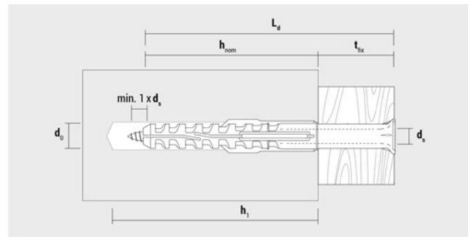
MFR 8: d_0 = 6 mm, MFR 10: d_0 = 7 mm, MFR 14: d_0 = 10 mm
